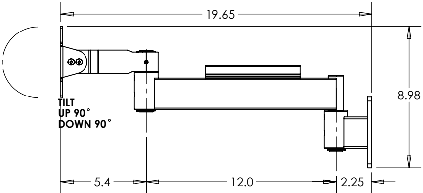
EXTENDED VIEW
