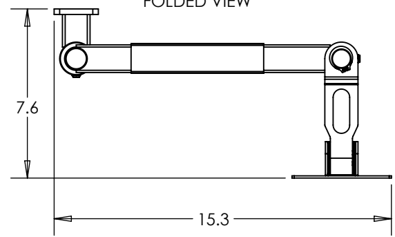
FOLDED VIEW
